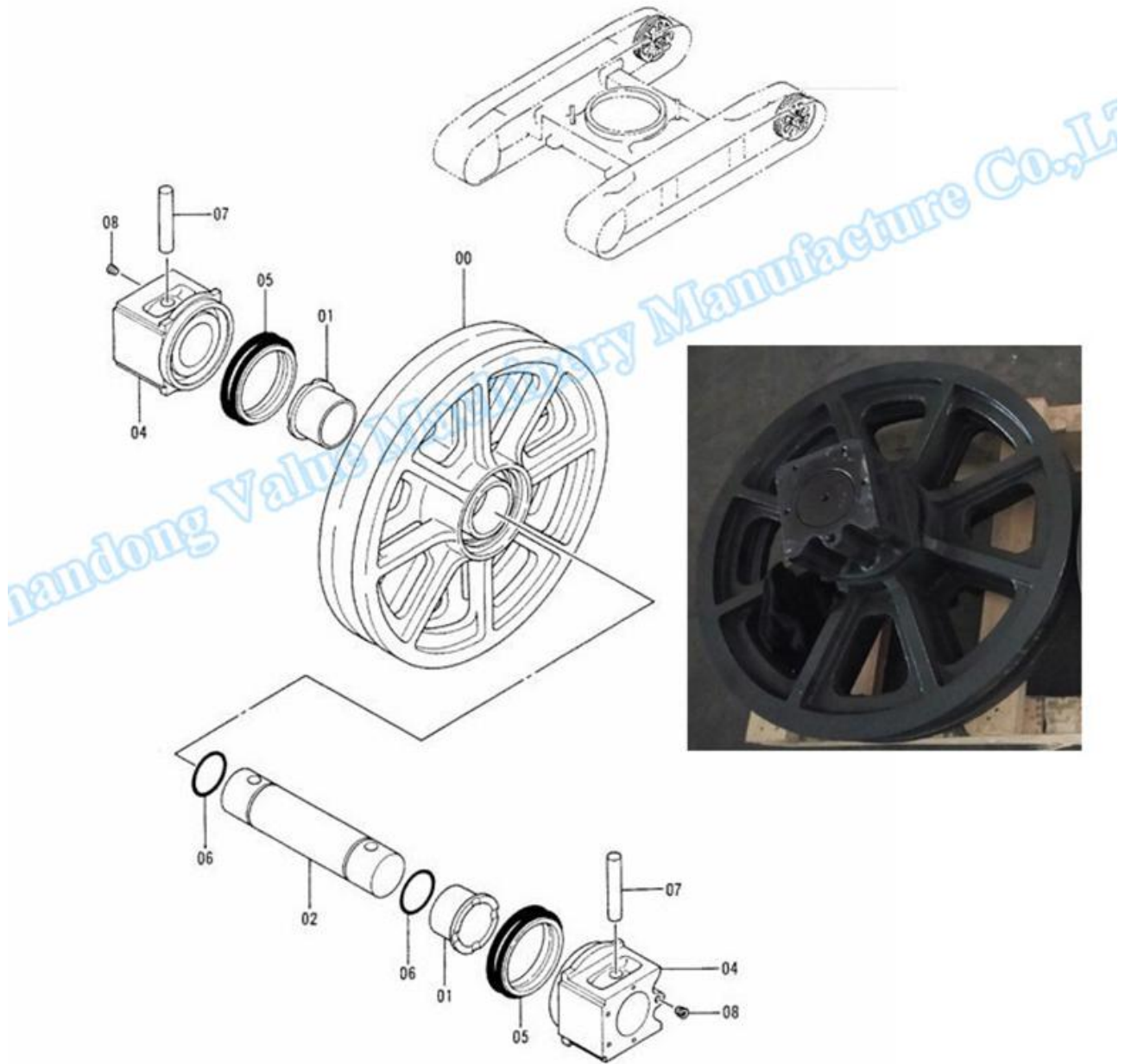
FRONT IDLER
