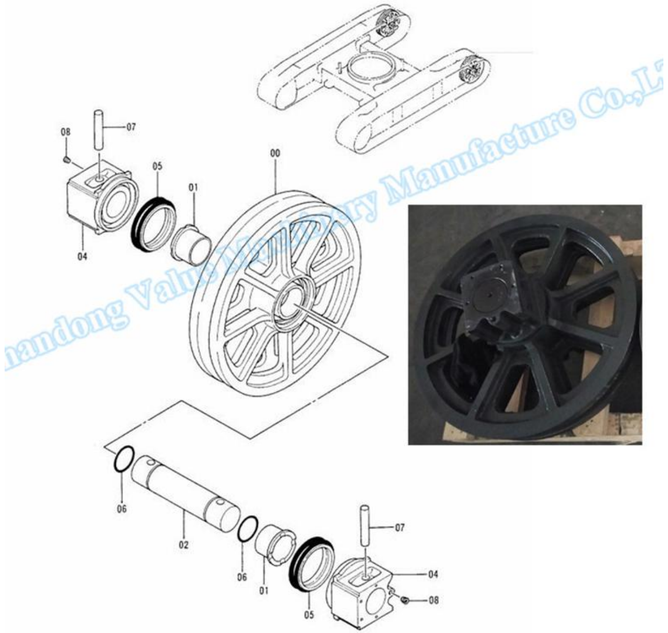
FRONT IDLER
